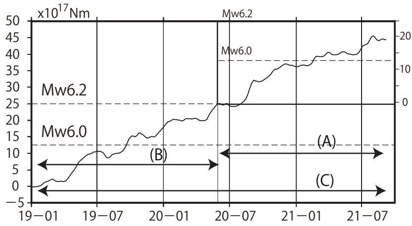
(A) 2020/6/1-2021/9/7 (今回)
