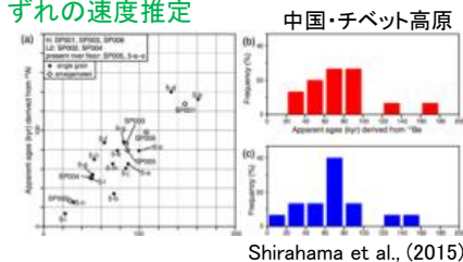
Shirahama et al., (2015)
