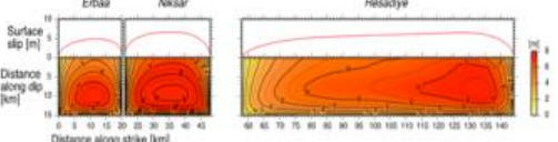
Kondo et al., JGR, (2010), Kase et al. (in prep.)
